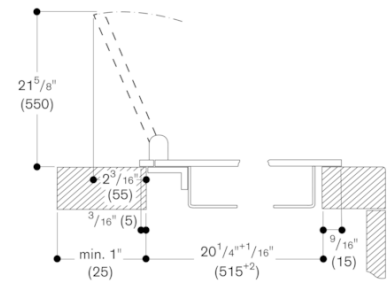
Installation with appliance cover/spacer batten; surface installation
