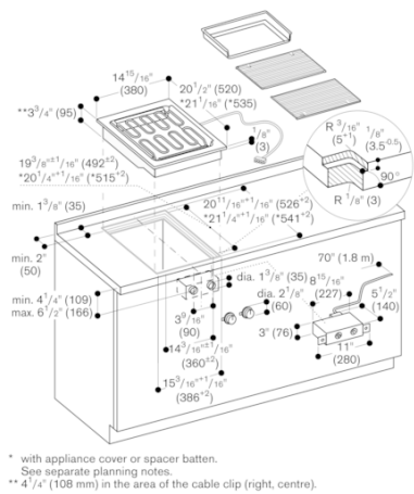
Installation with appliance cover/spacer batten; surface installation
