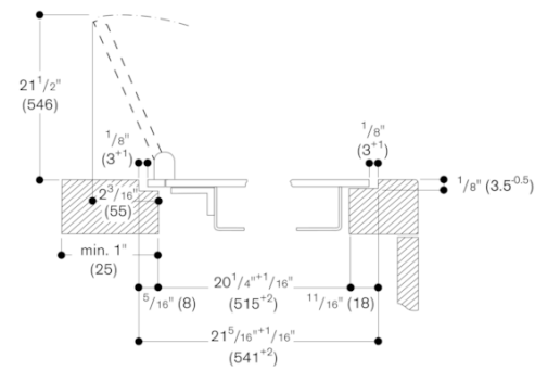
Installation with appliance cover/spacer batten; flush installation
