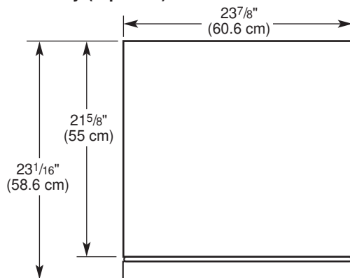
Style 2 - Overlay (top view)
