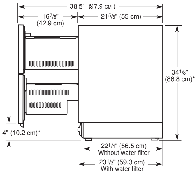
Style 2 - Overlay (side view)
